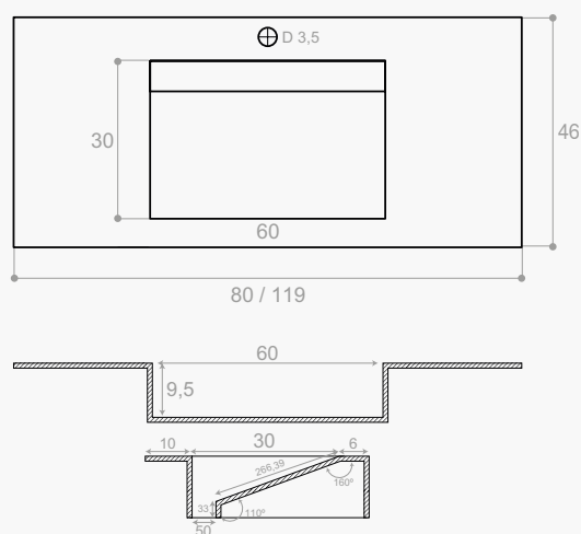
Tapa con lavabo integrado / Top with integrated basin
